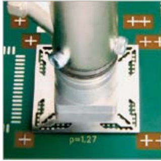
BGA
